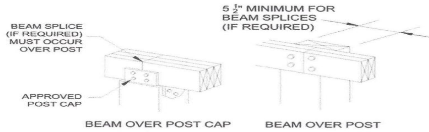
FIGURE R507.5.1(1) DECK BEAM TO DECK POST
